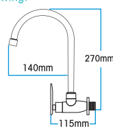
Sinor Handle Kitchen Sink Tap (Wall Mounted)
