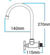
Cross Handle Kitchen Sink Tap (Wall Mounted)
