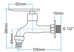
Sinor Handle Wall Bib Tap With Hose Connector
