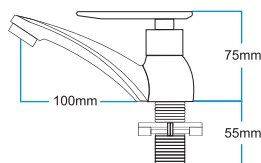
Sinor Handle Basin Tap – Pillar
