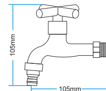
Cross Handle Wall Bib Tap With Hose Connector
